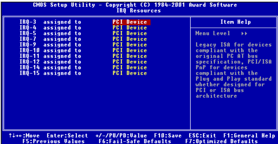
Figure 3-8B. IRQ Resources Menu
